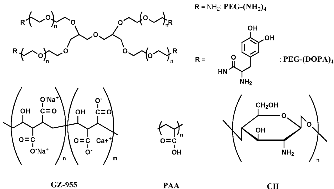
Fig. 1. Chemical structures of PEG-(NH 2 ) 4 , PEG-(DOPA) 4 , GZ-955, PAA, and CH.
