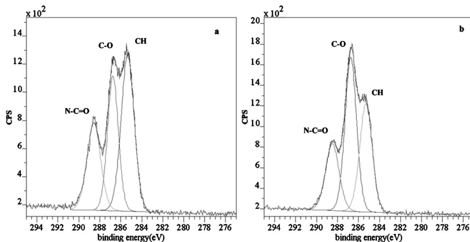
FIG. 3. High resolution C 1s scans of (a) \text{TiO}_2 coated Si wafer with adsorbed mucin and (b) \text{TiO}_2 coated Si wafer with adsorbed mucin and adsorbed PEG-(DOPA) 4 .
