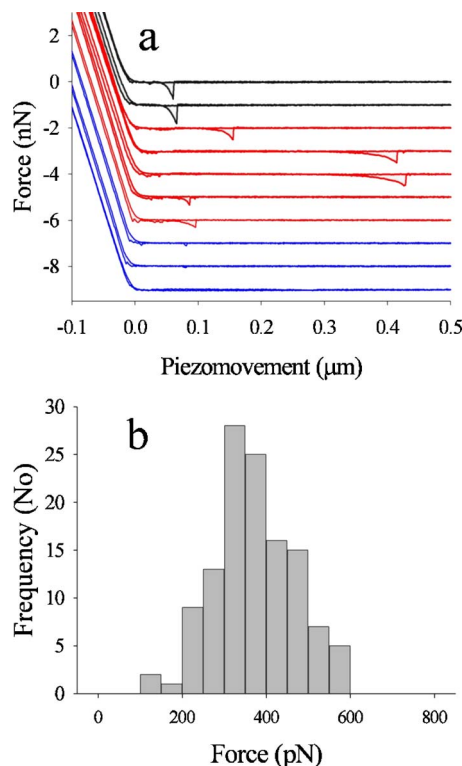
FIG. 9. Single molecule AFM results for interaction of DOPA with mucin. (a) Representative force-distance curves of DOPA-mucin interaction at \text{pH} of 7.4. The AFM cantilever was first confirmed to contain PEG tethered N -Boc-DOPA by obtaining F - D curves on \text{TiO}_2 (black), revealing the expected \sim 800 pN pull-off force (Ref. 29). After changing the substrate to mucin coated \text{TiO}_2 , DOPA-mucin interactions were revealed by force signals observable at pull-off distances of up to 400 nm or more (red). DOPA free control AFM cantilevers prepared with methoxy terminated PEG showed only weak interactions with mucin (blue). (b) Force histogram of DOPA-mucin interaction force. Statistical analysis revealed an average force value of 371 \pm 98 pN ( n=121 , pooled data for all \text{pH} values tested).
