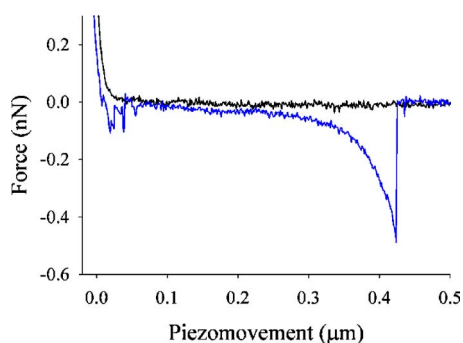
FIG. 10. Detailed example of F-D curve showing approach (black) and retraction (blue) for interaction of DOPA with mucin at pH of 7.4. The retraction curve deviated from the approach curve beginning at short distances and culminated in separation of DOPA from mucin at an extension of greater than 400 nm, after which the force returned to zero.
