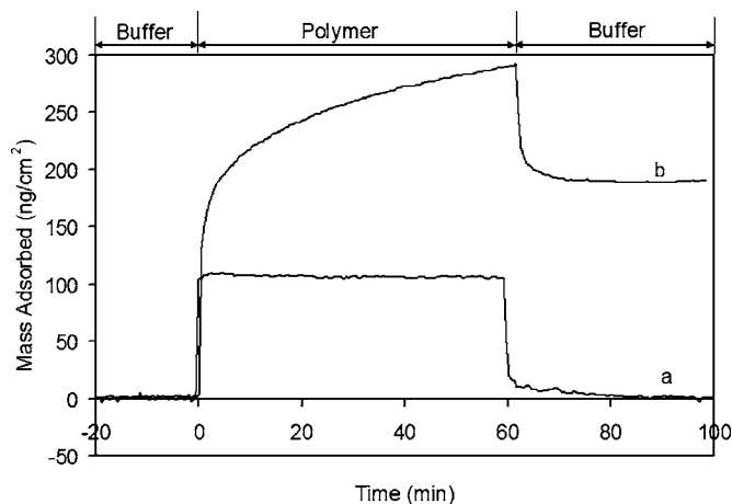
FIG. 5. OWLS traces showing mass adsorbed vs time for interaction of a solution containing (a) PEG-(NH 2 ) 4 and (b) PEG-(DOPA) 4 with a mucin coated TiO 2 waveguide. The polymer solution concentration in both cases was 10 mg/mL in 10 mM HEPES, pH of 7.4.
