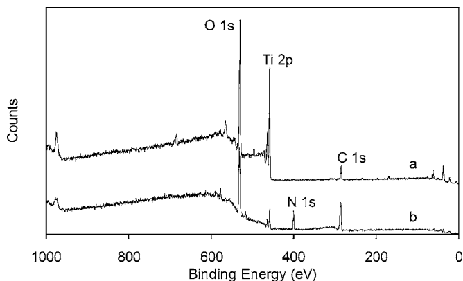
FIG. 2. XPS survey scans of (a) \text{TiO}_2 coated Si wafer and (b) \text{TiO}_2 coated Si wafer with adsorbed mucin.
