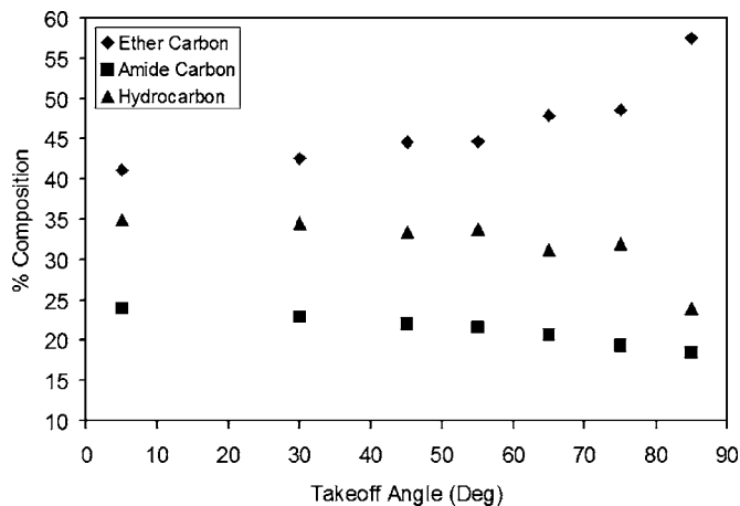
FIG. 4. Percent composition of XPS C 1s peak components vs takeoff angle for the case of PEG-(DOPA) 4 adsorbed to a mucin layer on a \text{TiO}_2 coated Si wafer.
